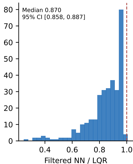
Attitude RMS ratio
