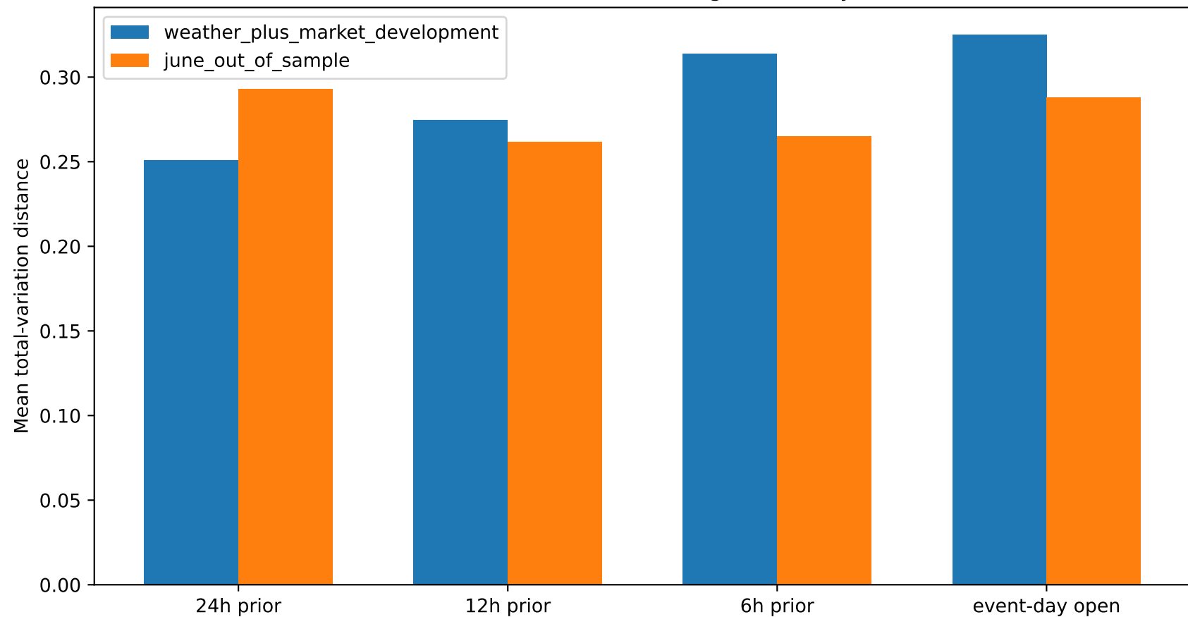
GP-market distributional disagreement by rule
