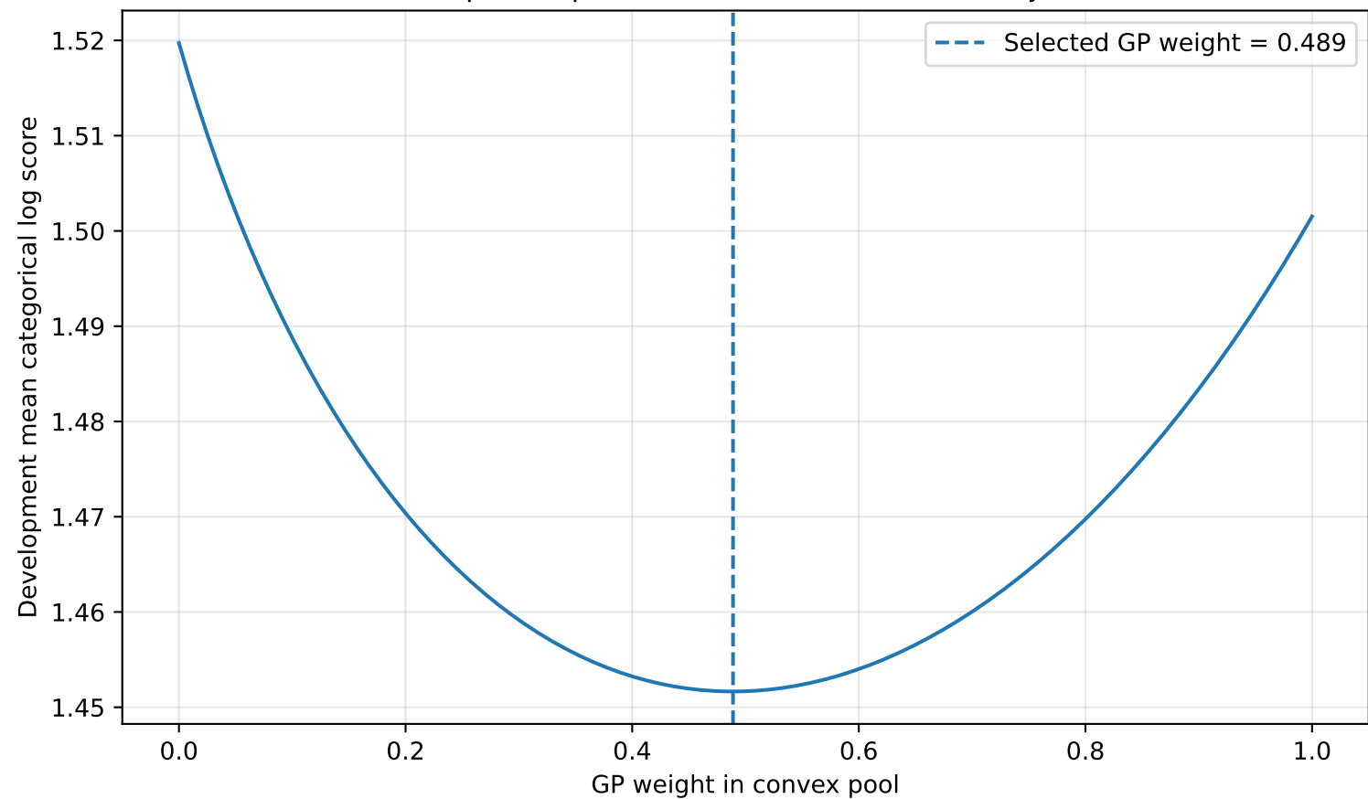
Development-period forecast-combination objective
