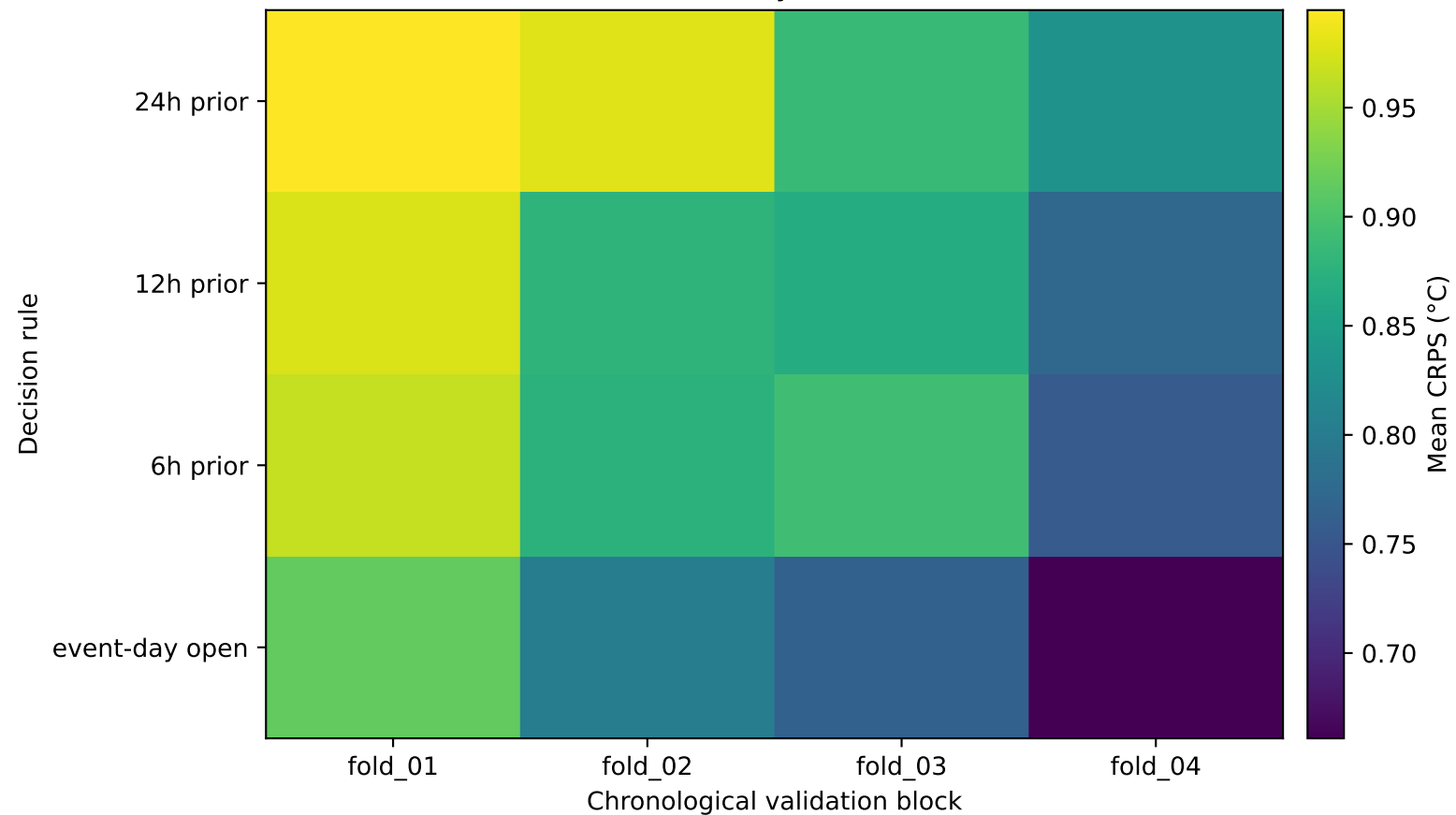
Matérn-3/2 mean CRPS by decision rule and block
