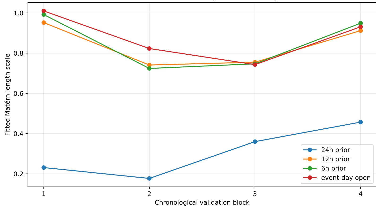
Fold-to-fold Matérn length-scale stability
