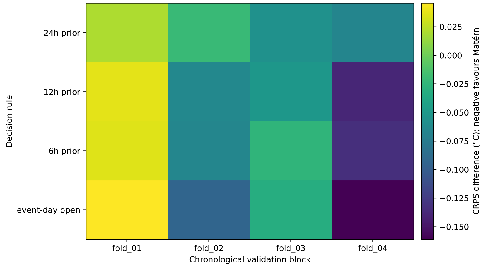
Matérn-3/2 minus static Gaussian mean CRPS
