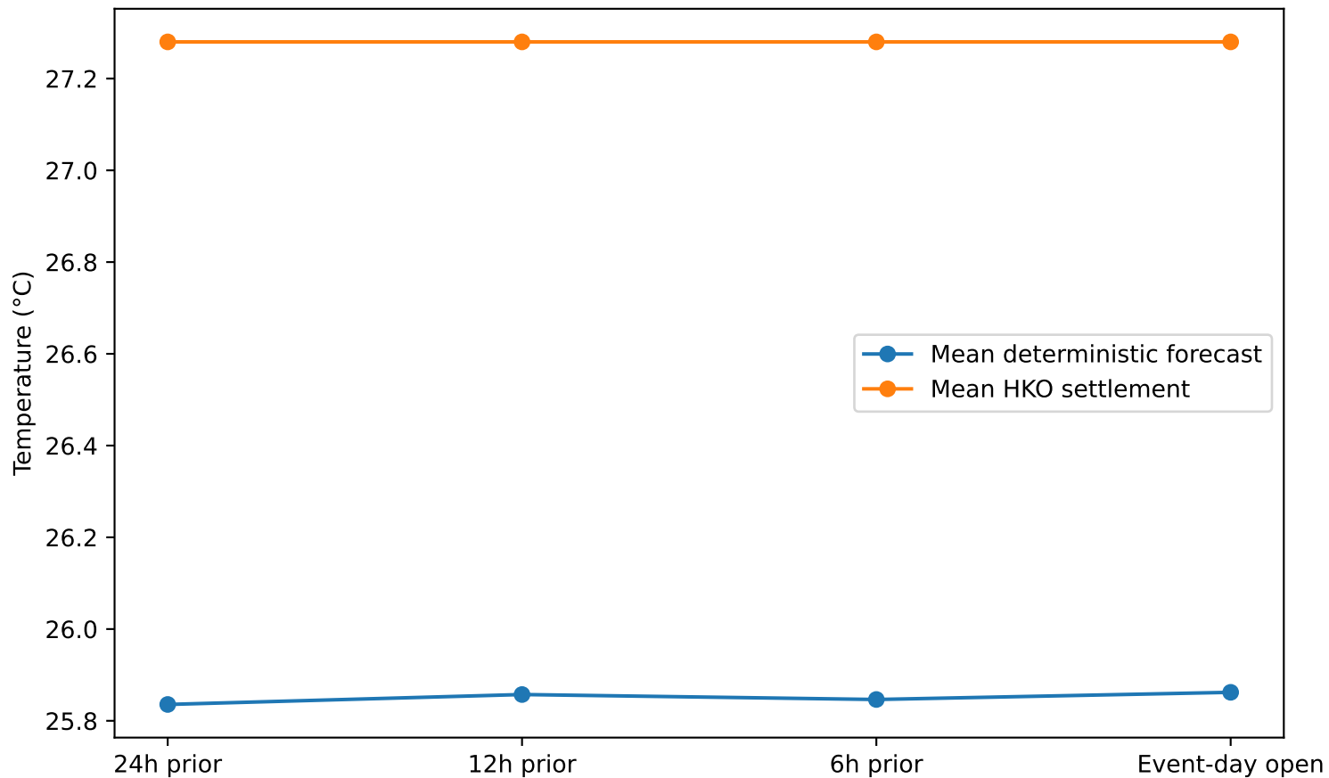
Forecast level across decision rules
