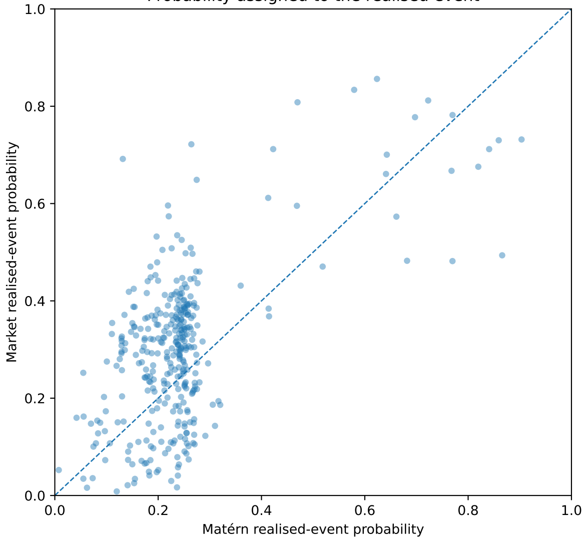
Probability assigned to the realised event
