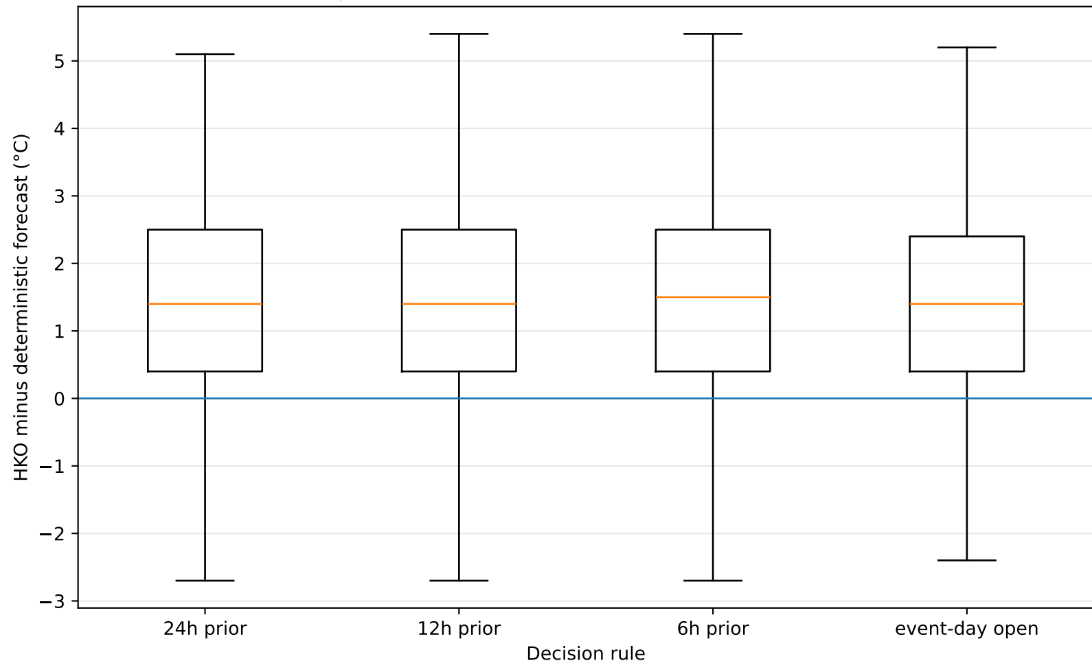
Rule-specific deterministic forecast errors over 730 dates
