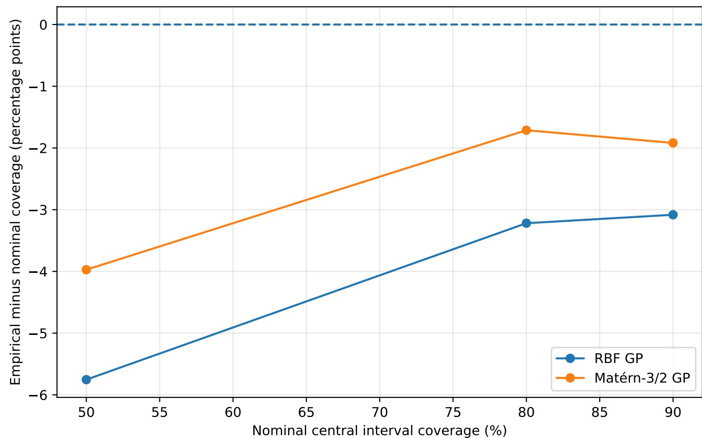
Central-interval calibration
