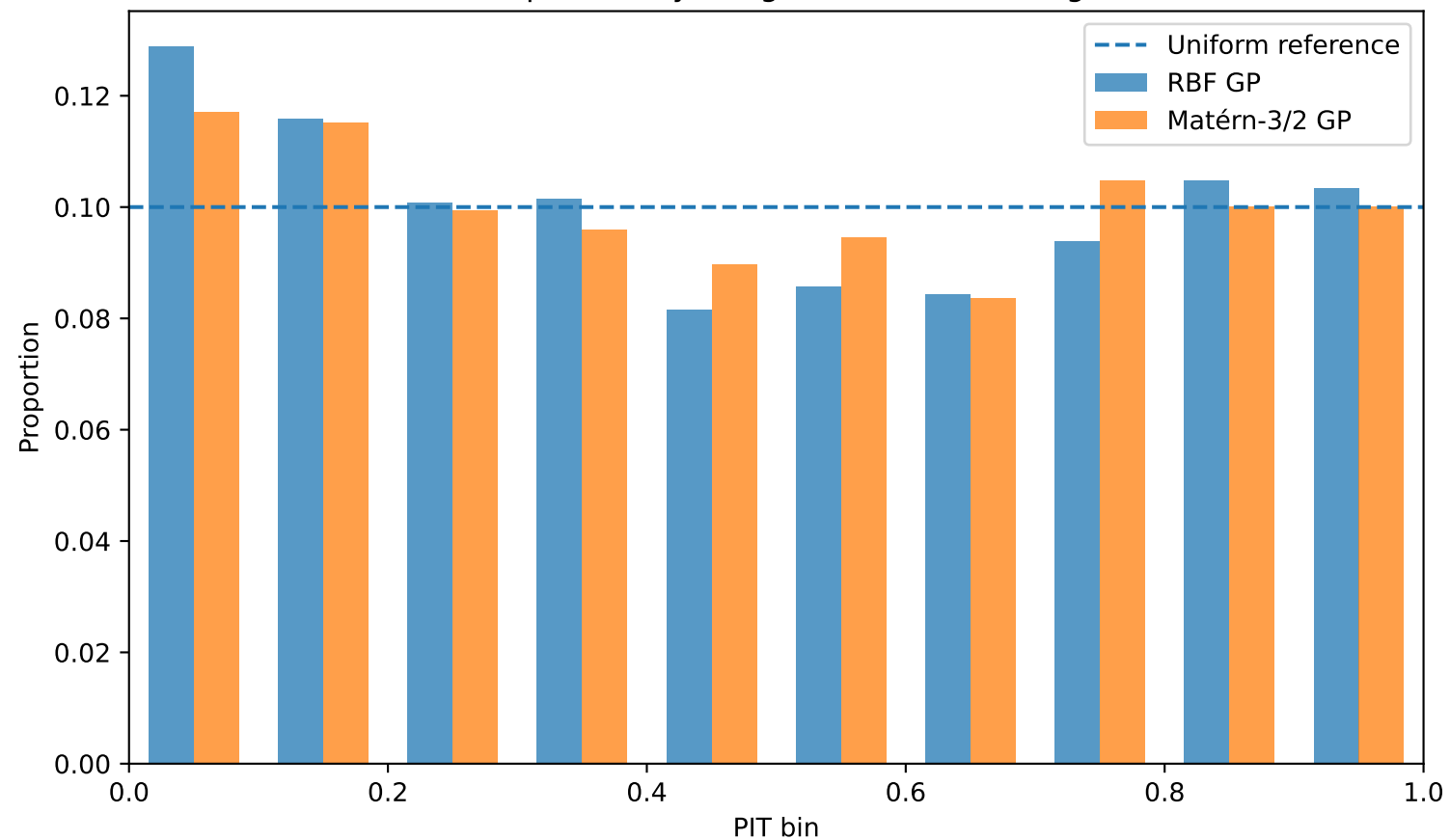
Overall probability integral transform histogram
