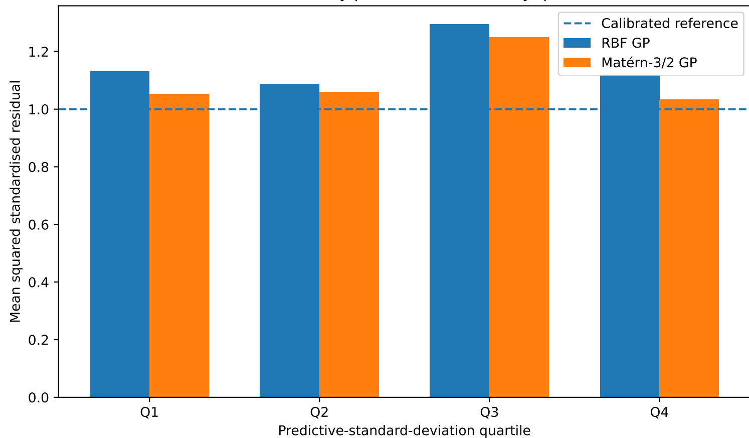
Residual scale by predictive-uncertainty quartile
