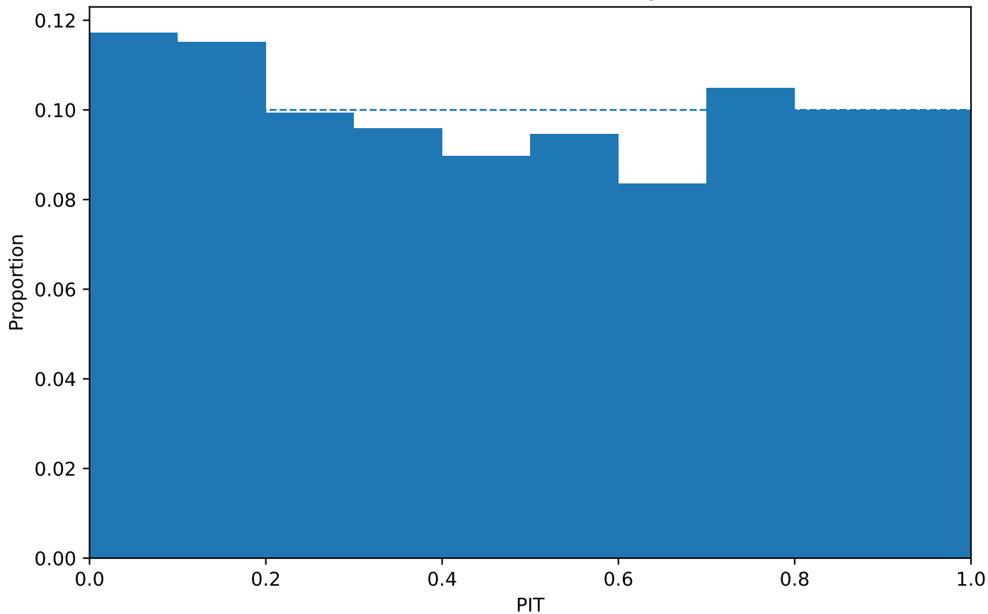
Selected Matérn PIT histogram
