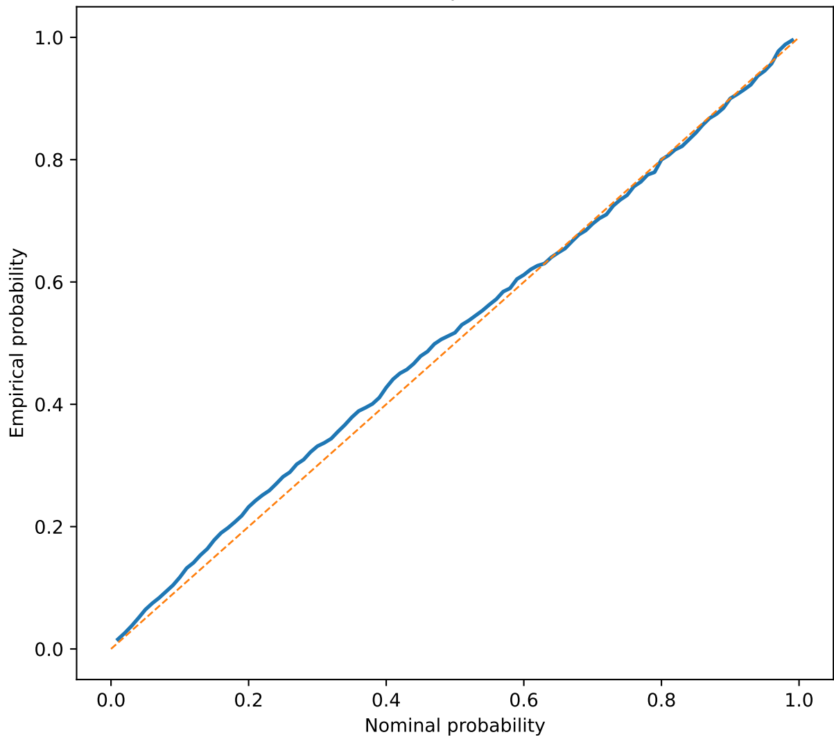
Selected Matérn quantile calibration
