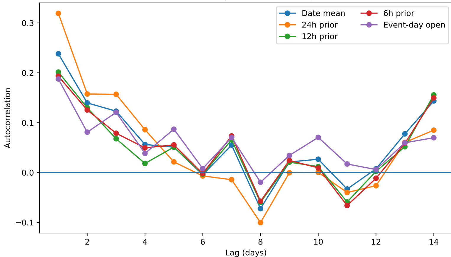
Selected Matérn squared-residual dependence
