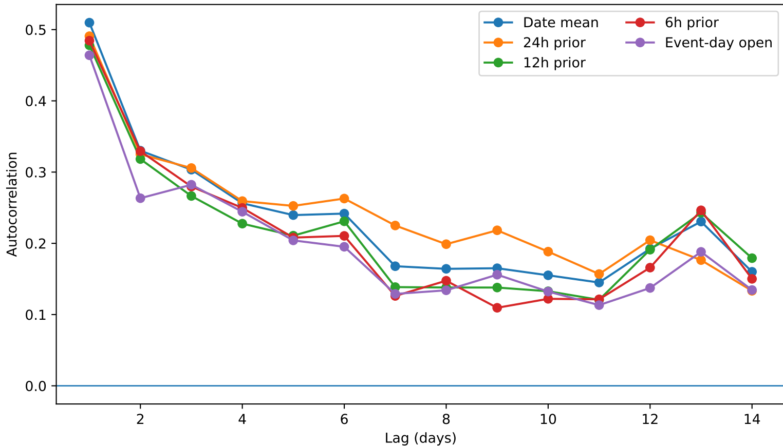
Selected Matérn standardised-residual dependence
