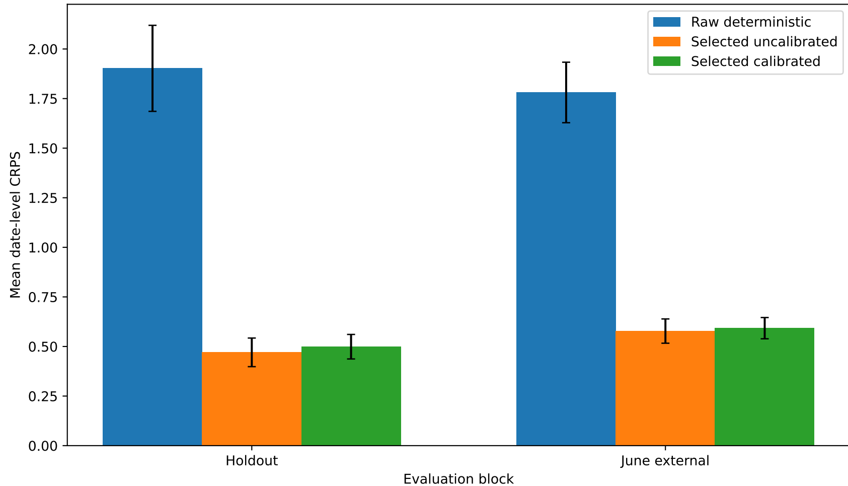
Locked continuous forecast performance
