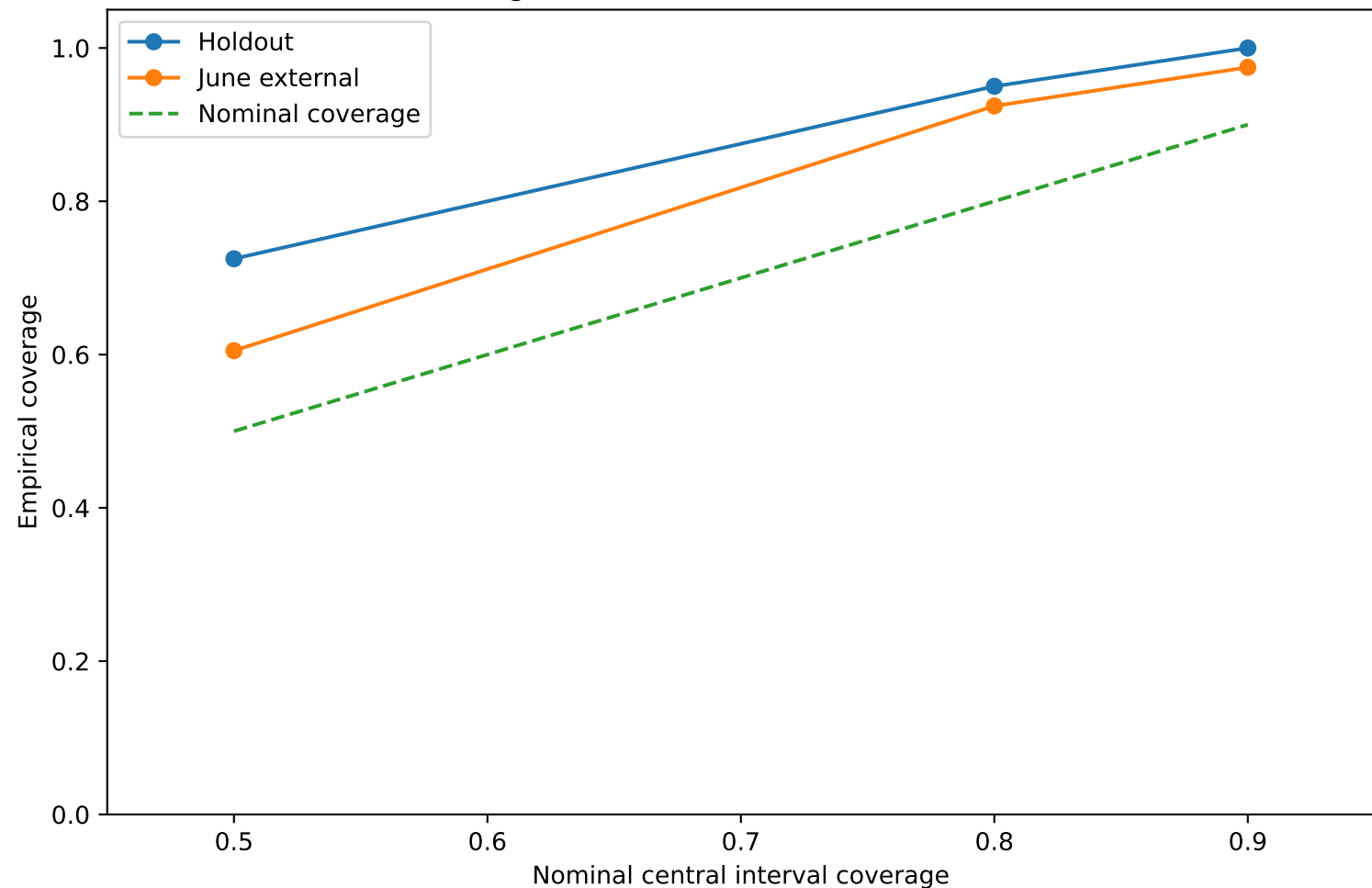
Coverage of the locked calibrated distribution
