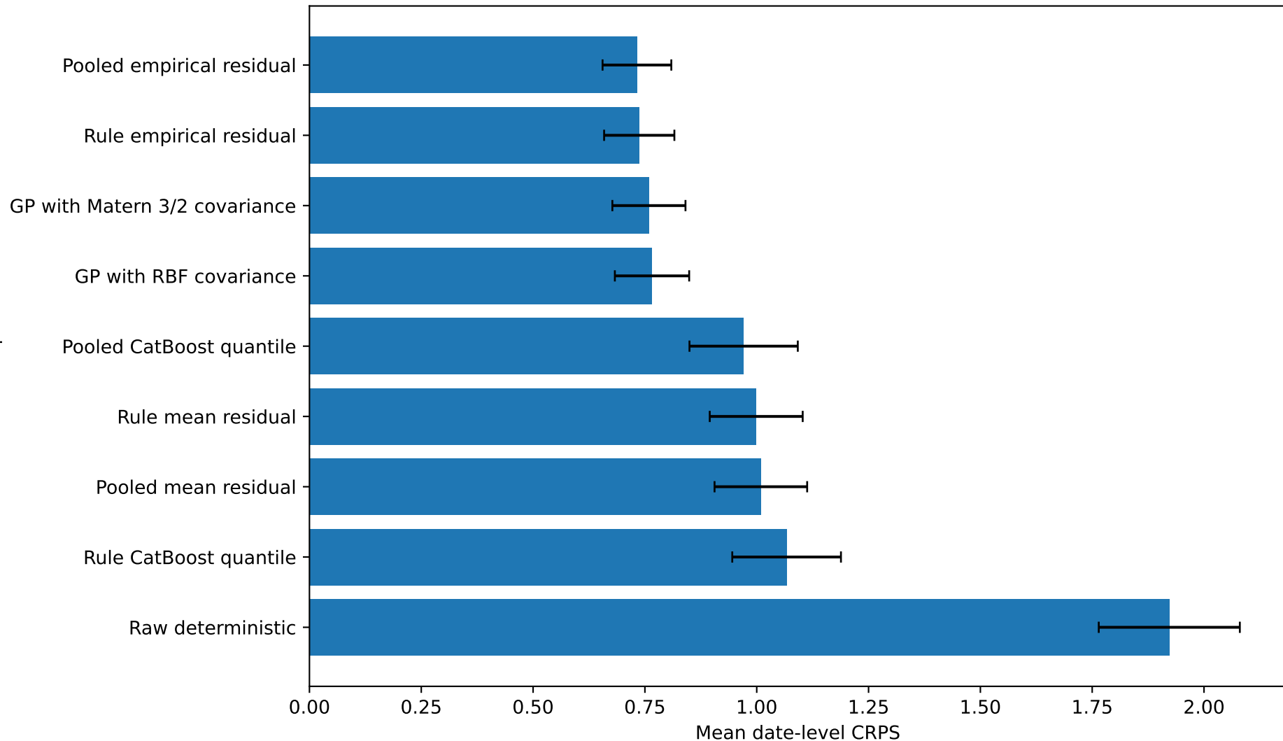
Chronological out-of-fold probabilistic forecast comparison
