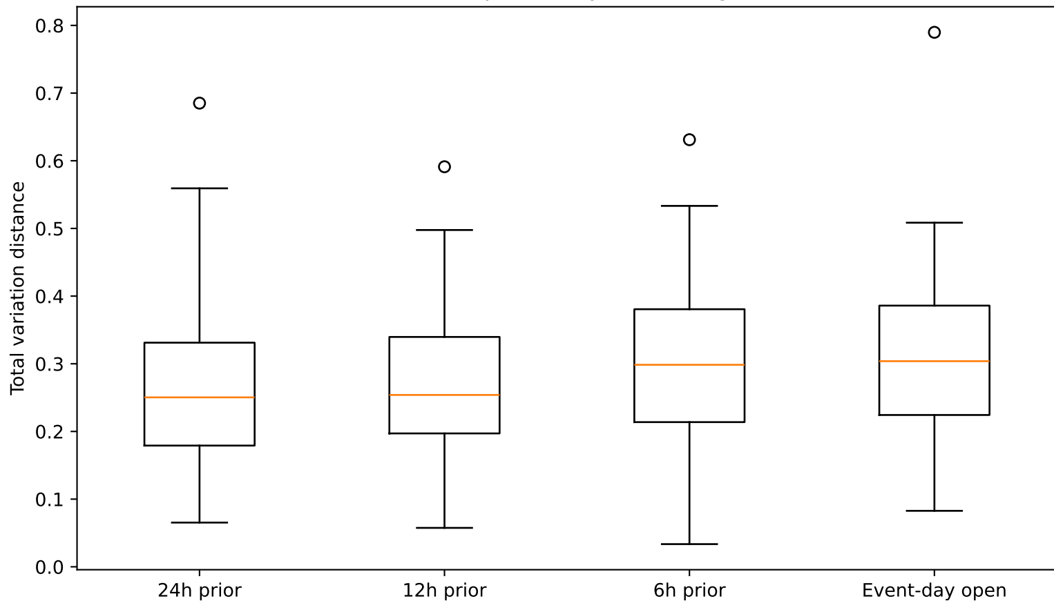
Matérn-market probability-book disagreement
