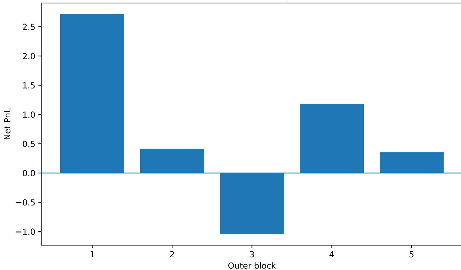
Nested walk-forward PnL by outer block
