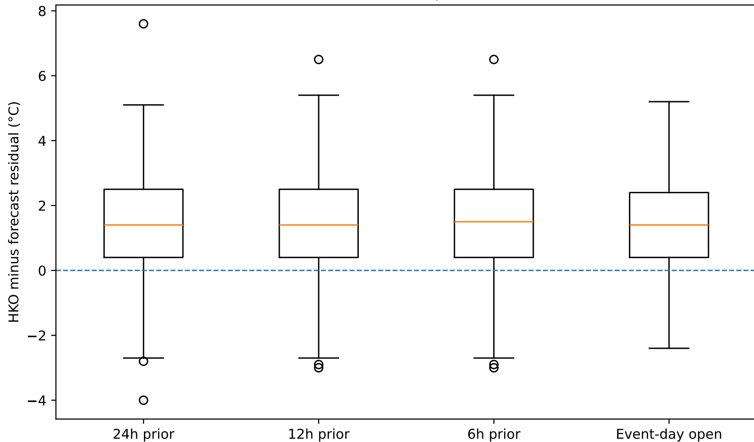
Settlement residual by decision rule
