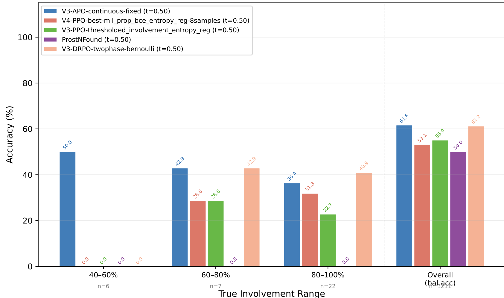
Accuracy by Involvement — csPCa (GG \geq 3) Classification Head [fixed t=0.50] (bins \geq 20%: cancer-only \rightarrow value = sensitivity at that level)
