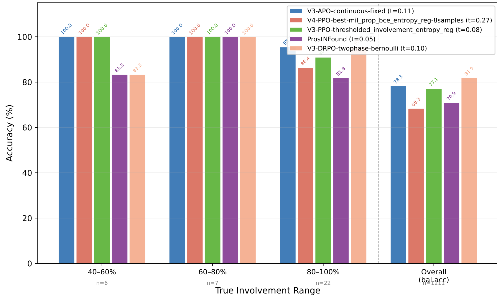
Accuracy by Involvement — csPCa (GG \geq 3) Classification Head [optimal t] (bins \geq 20%: cancer-only \rightarrow value = sensitivity at that level)
