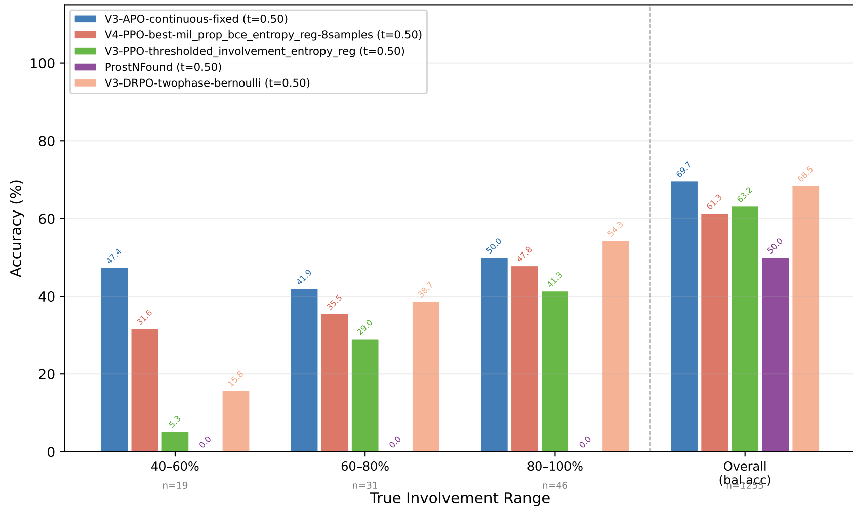
Accuracy by Involvement — High-Inv (>40%) Classification Head [fixed t=0.50 ] (bins \geq 20\% : cancer-only \rightarrow value = sensitivity at that level)
