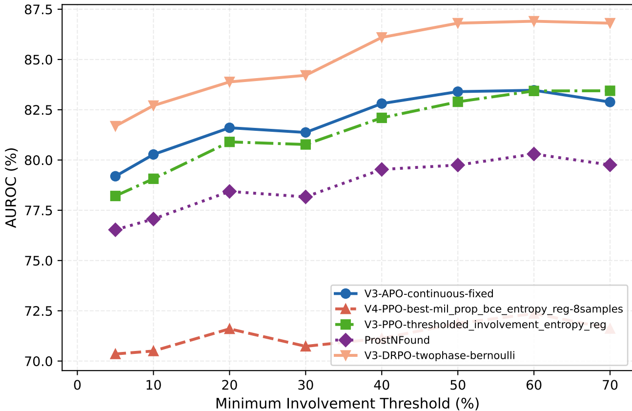
AUROC vs Involvement Threshold High-Inv (>40%) — Classification Head ( )
