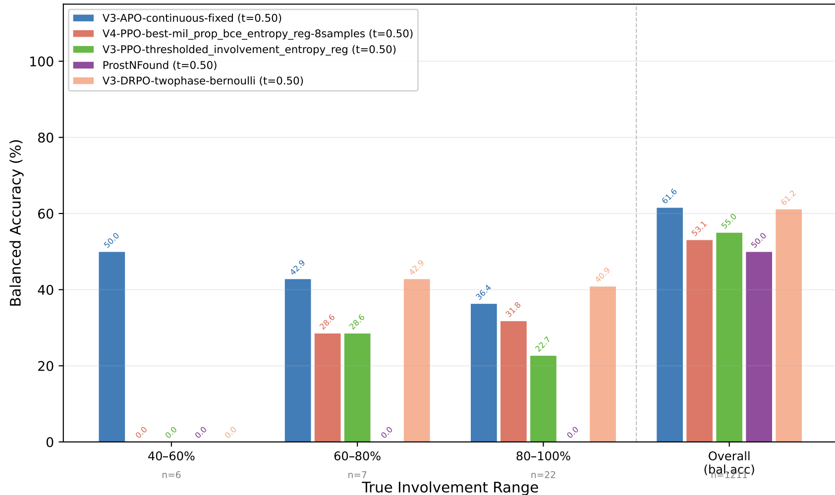
Balanced Accuracy by Involvement — csPCa (GG \geq 3) Classification Head [fixed t=0.50] (bins \geq 20%: cancer-only \rightarrow value = sensitivity at that level)
