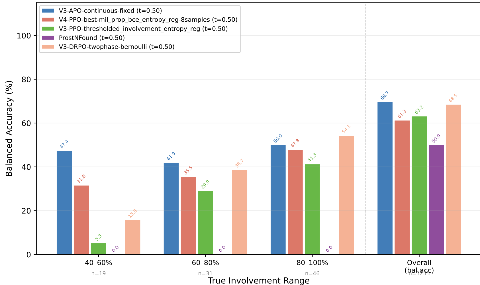
Balanced Accuracy by Involvement — High-Inv (>40%) Classification Head [fixed t=0.50 ] (bins \geq 20\% : cancer-only \rightarrow value = sensitivity at that level)
