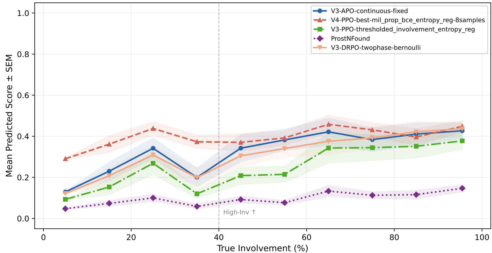
Prediction vs Involvement — Classification Head ( )
