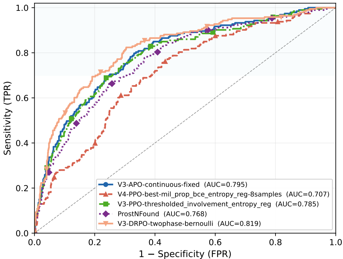
ROC — All Cores Classification Head
