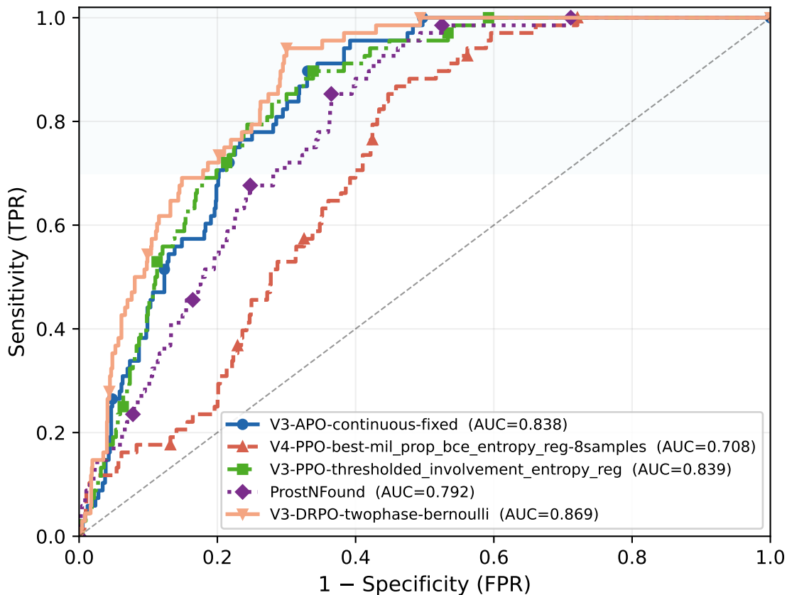
ROC — csPCa (GG \geq 3) Classification Head
