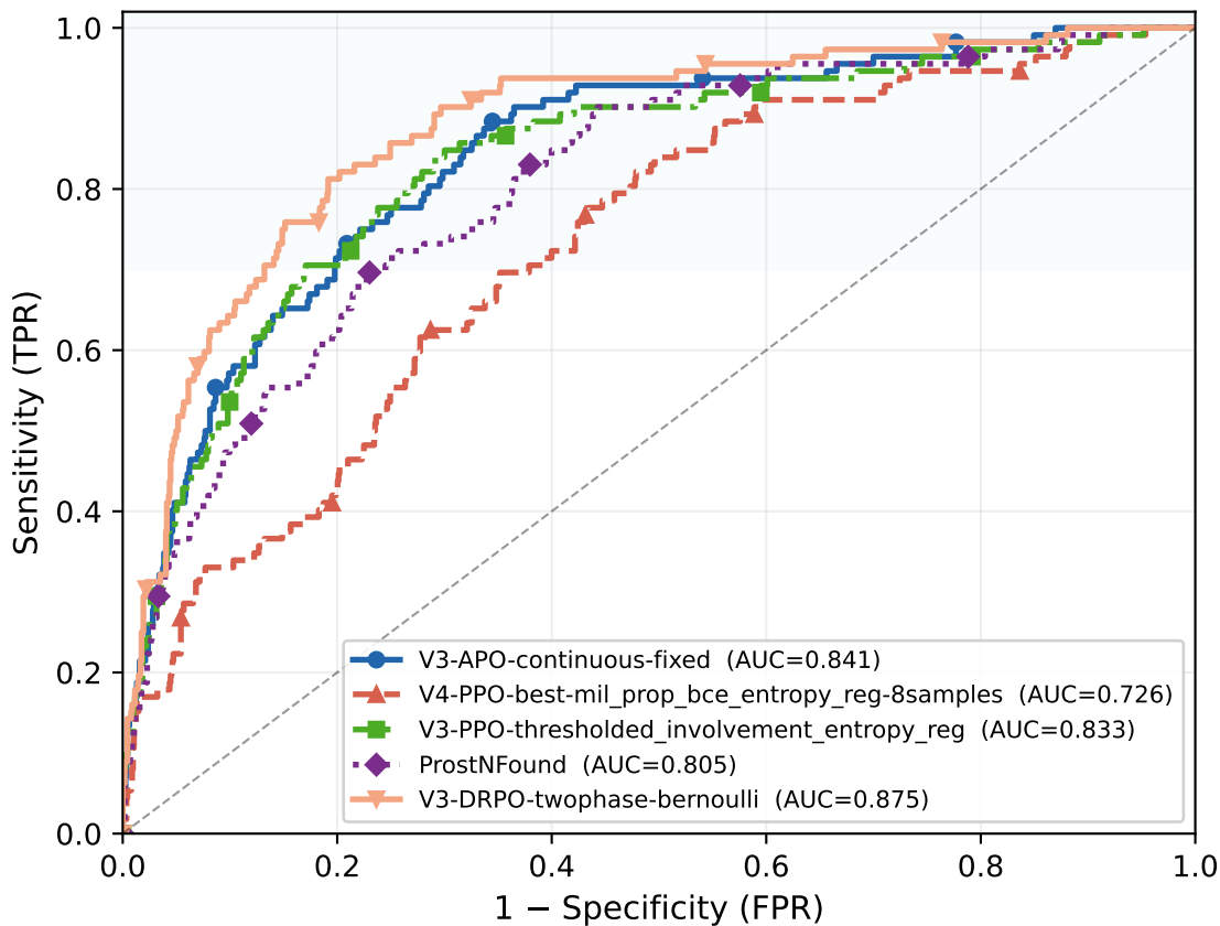
ROC — High-Inv (>40%) Classification Head
