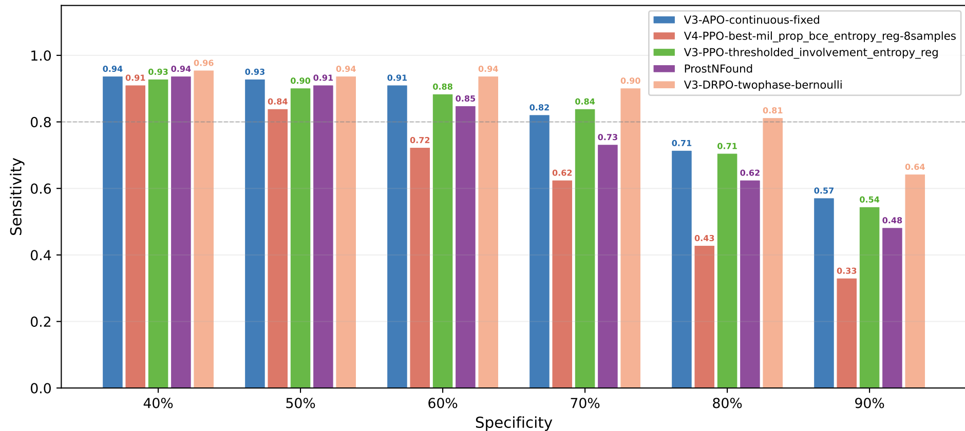
Sensitivity @ Specificity — High-Inv (>40%) Classification Head
