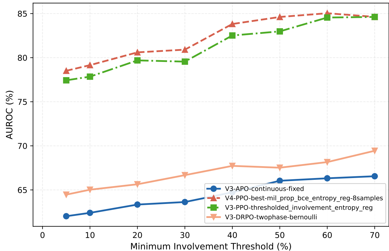
AUROC vs Involvement Threshold All Cores — Heatmap Head (Thresh.) (thresholded)
