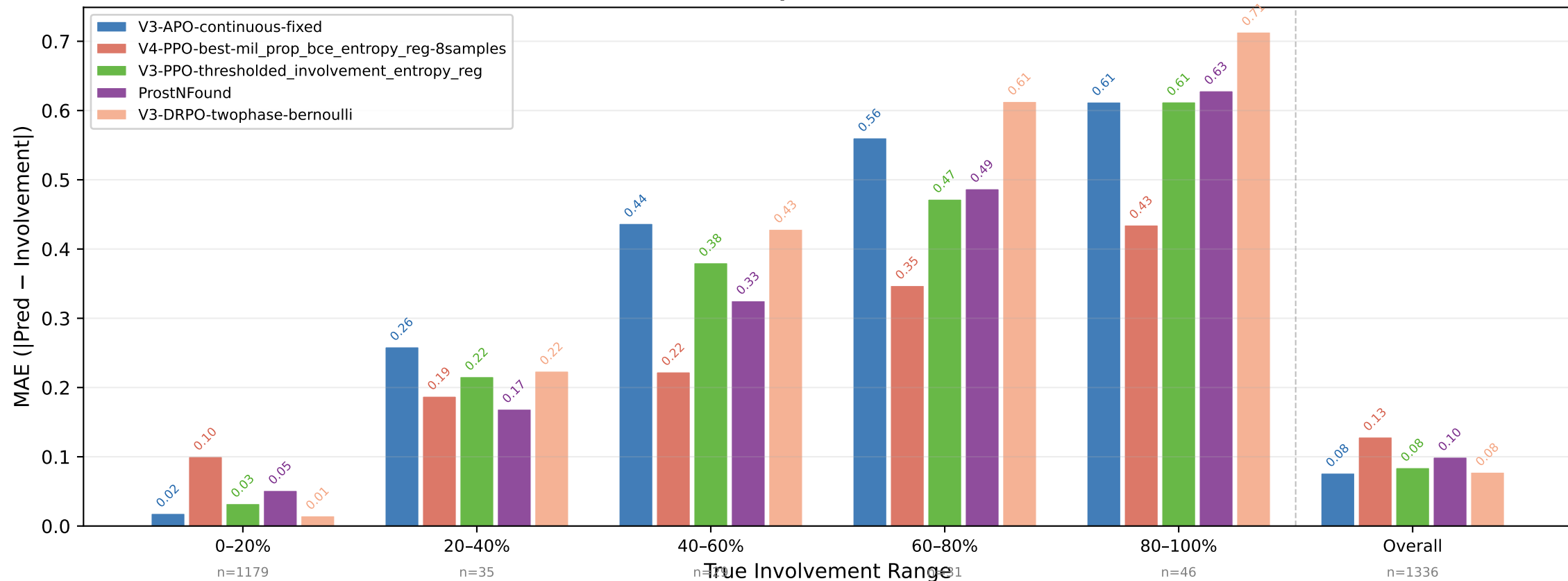
Error by Involvement — All Cores Heatmap Head (normal)
