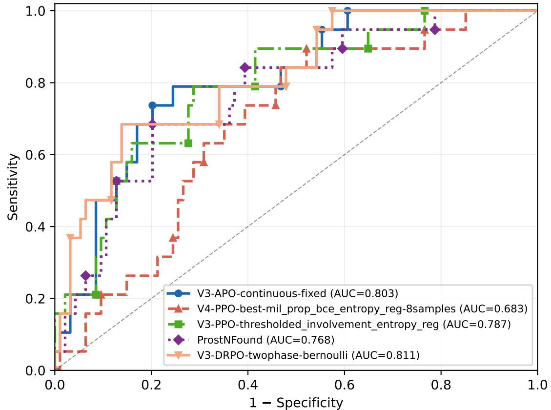
Patient-Level ROC — csPCa Patients (GG \geq 3) Classification Head (max score)
