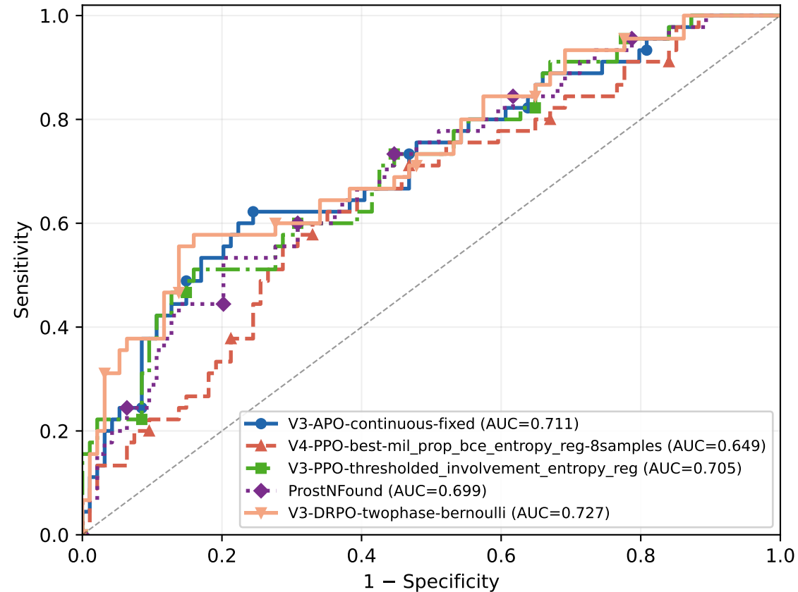
Patient-Level ROC — All Patients Classification Head (max score)
