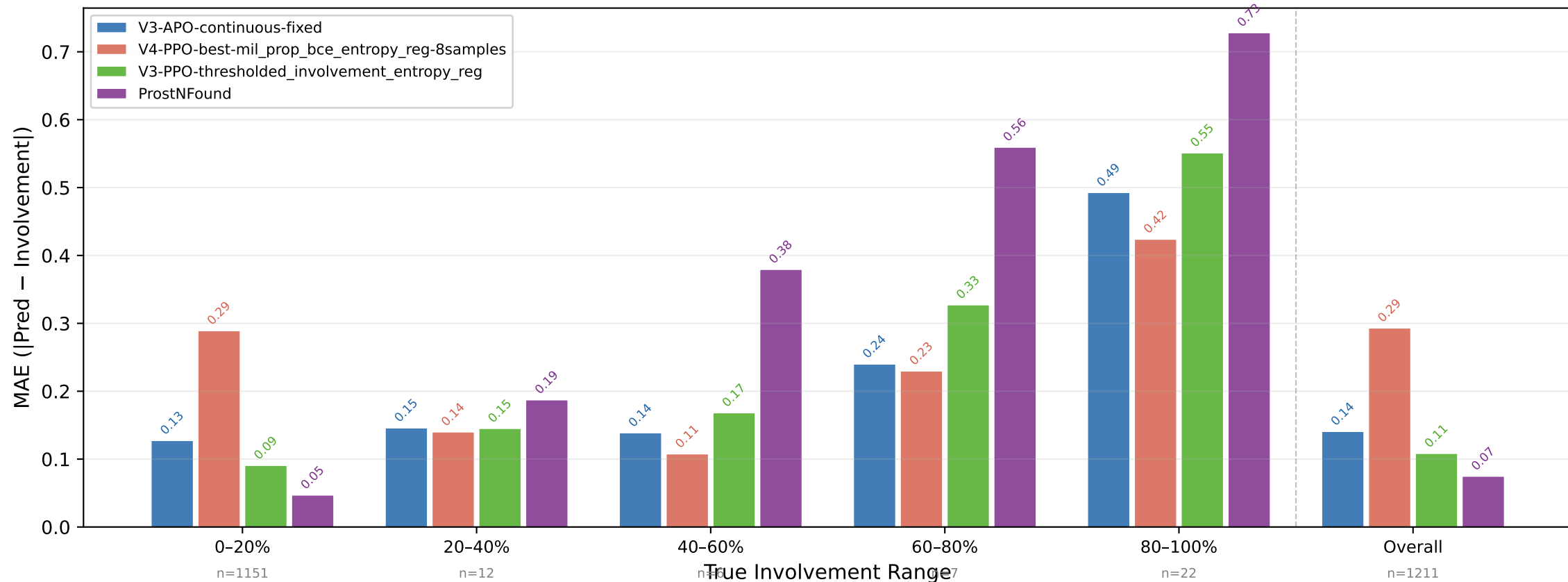
Error by Involvement — csPCa (GG \geq 3) Classification Head ( )
