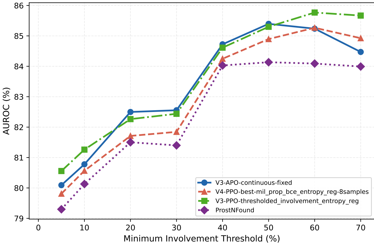
AUROC vs Involvement Threshold All Cores — Heatmap Head (normal)
