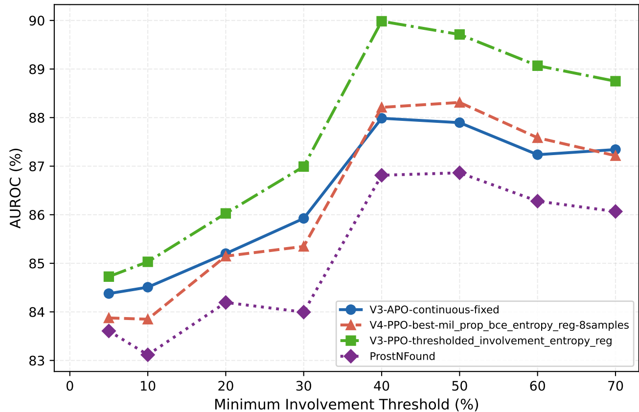
AUROC vs Involvement Threshold csPCa (GG \geq 3) — Heatmap Head (normal)
