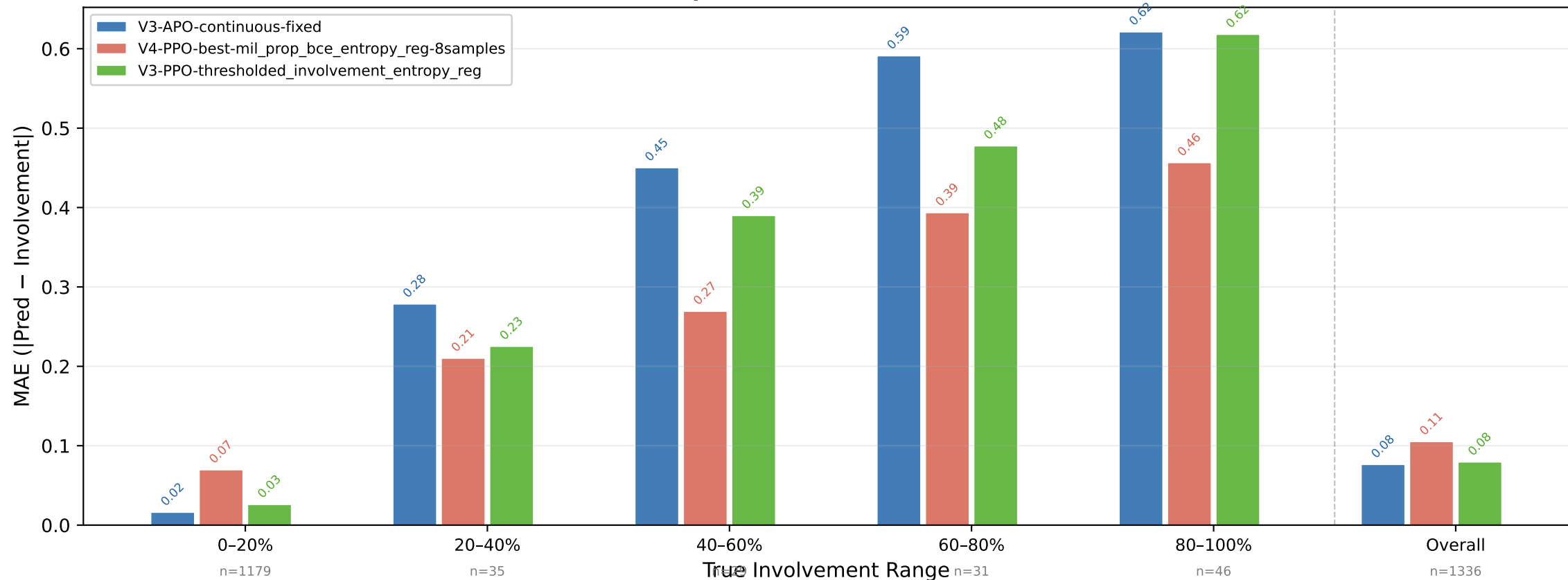
Error by Involvement — All Cores Heatmap Head (Thresh.) (thresholded)
