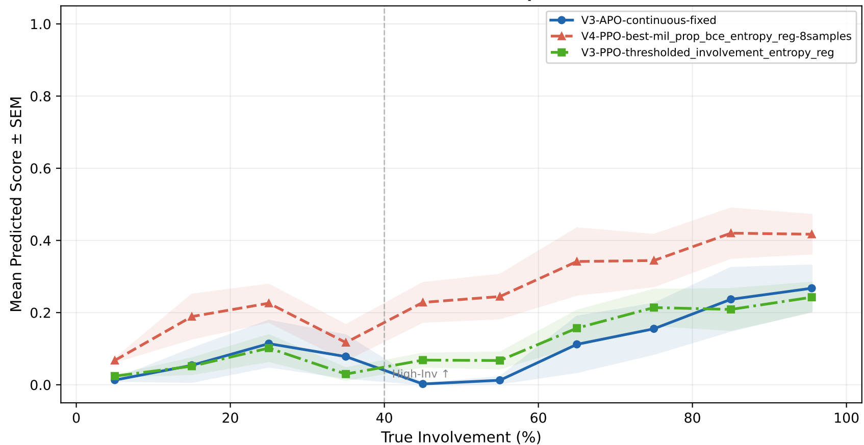
Prediction vs Involvement — Heatmap Head (thresholded)
