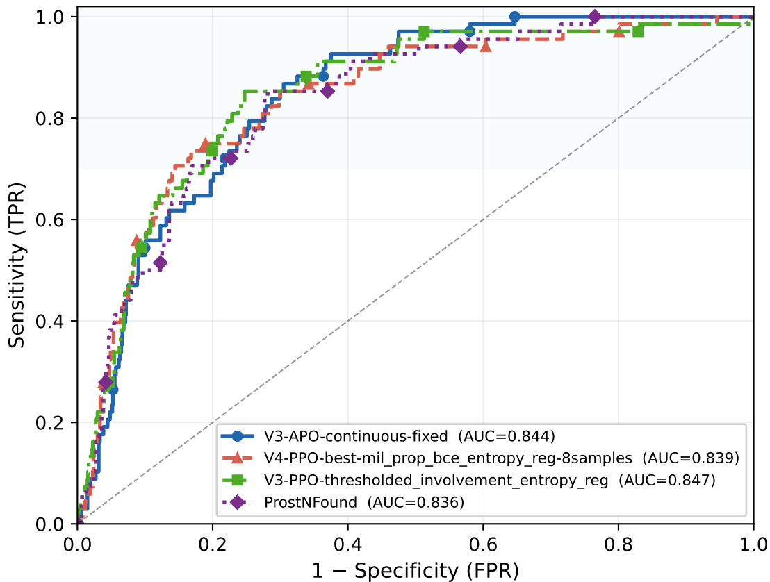
ROC — csPCa (GG \geq 3) Heatmap Head
