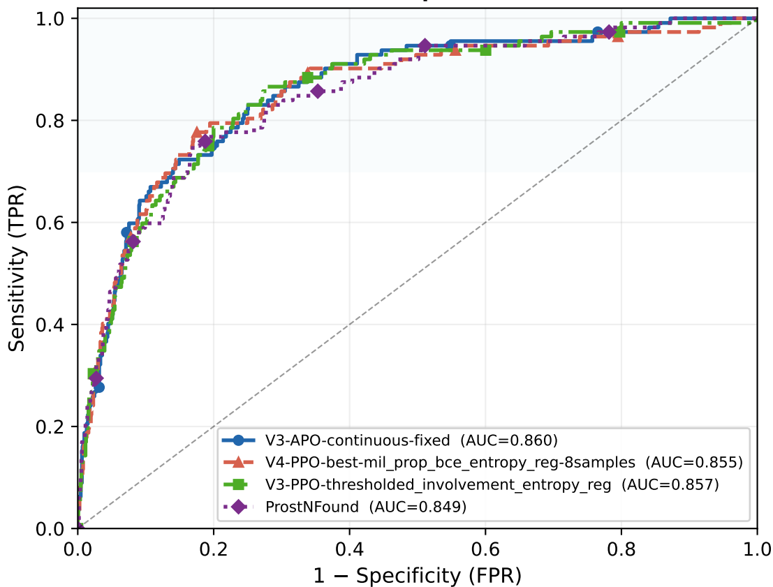
ROC — High-Inv (>40%) Heatmap Head
