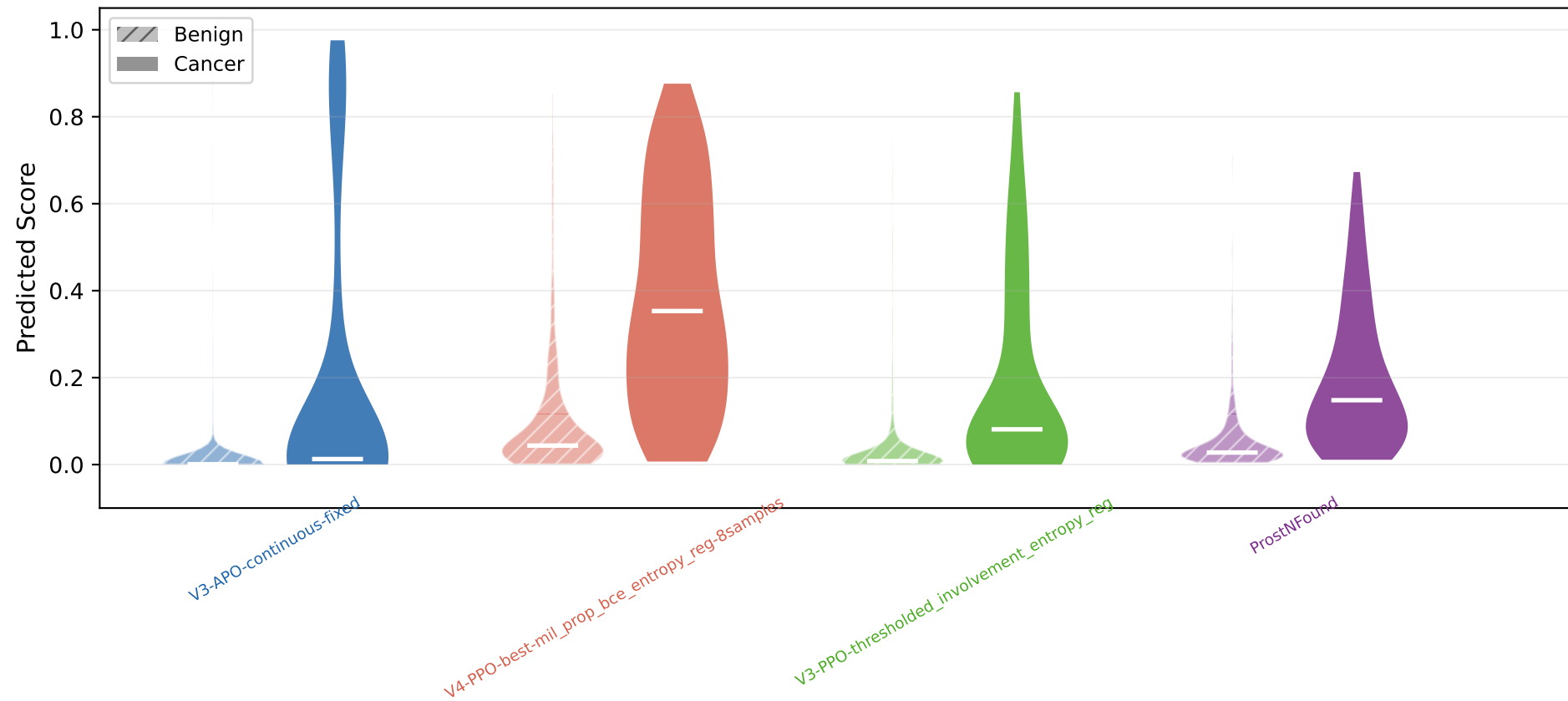
Score Distributions — High-Inv (>40%) Heatmap Head
