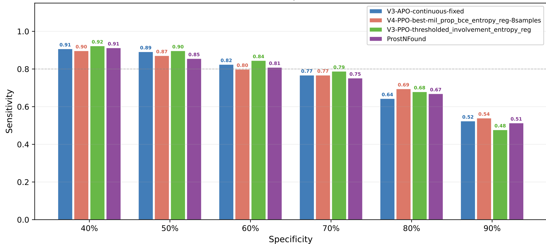
Sensitivity @ Specificity — All Cores Heatmap Head
