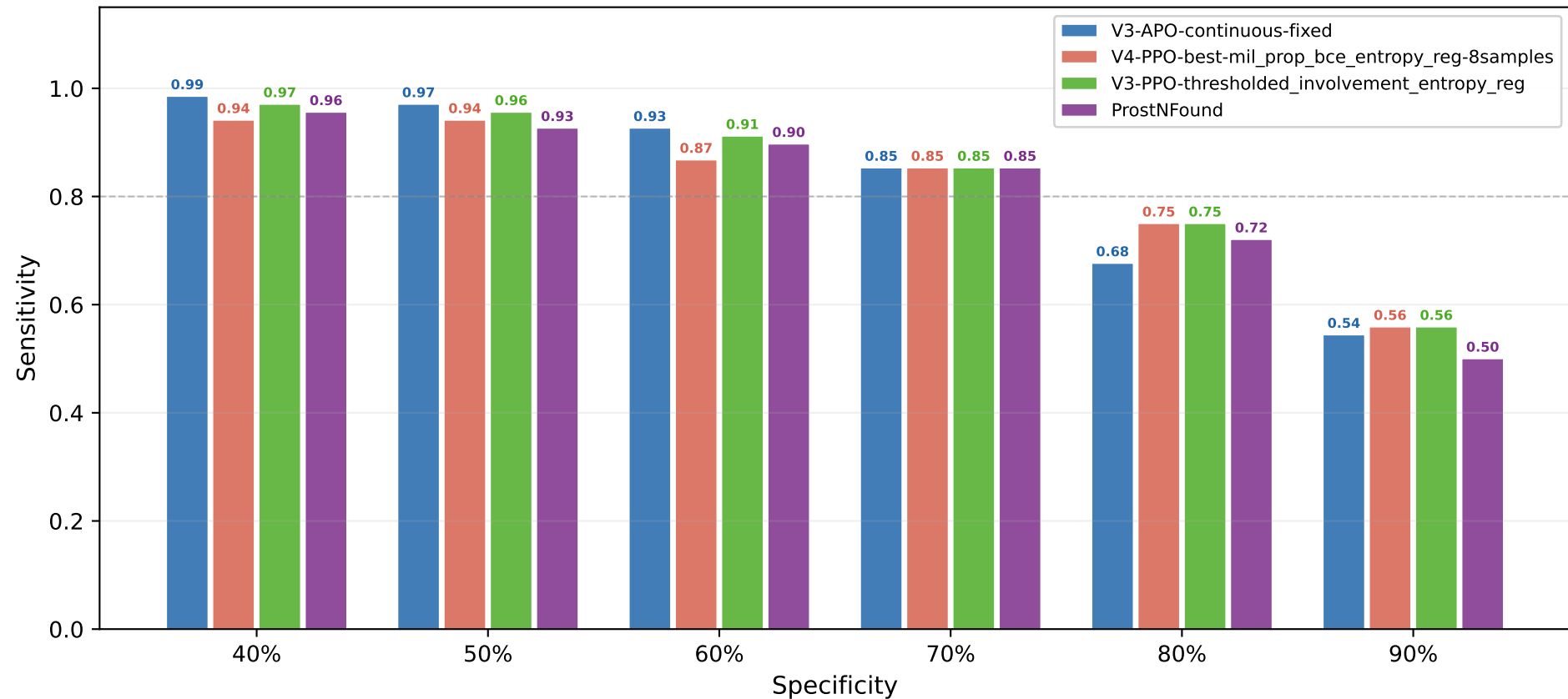
Sensitivity @ Specificity — csPCa (GG \geq 3) Heatmap Head
