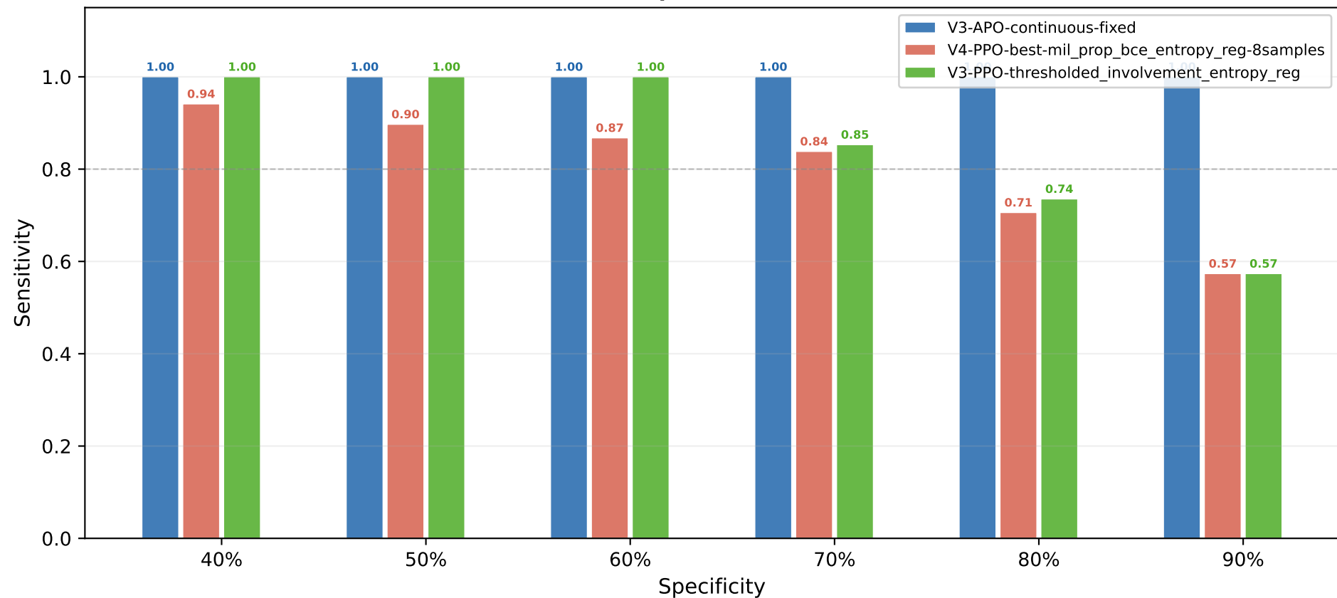
Sensitivity @ Specificity — csPCa (GG \geq 3) Heatmap Head (Thresh.)
