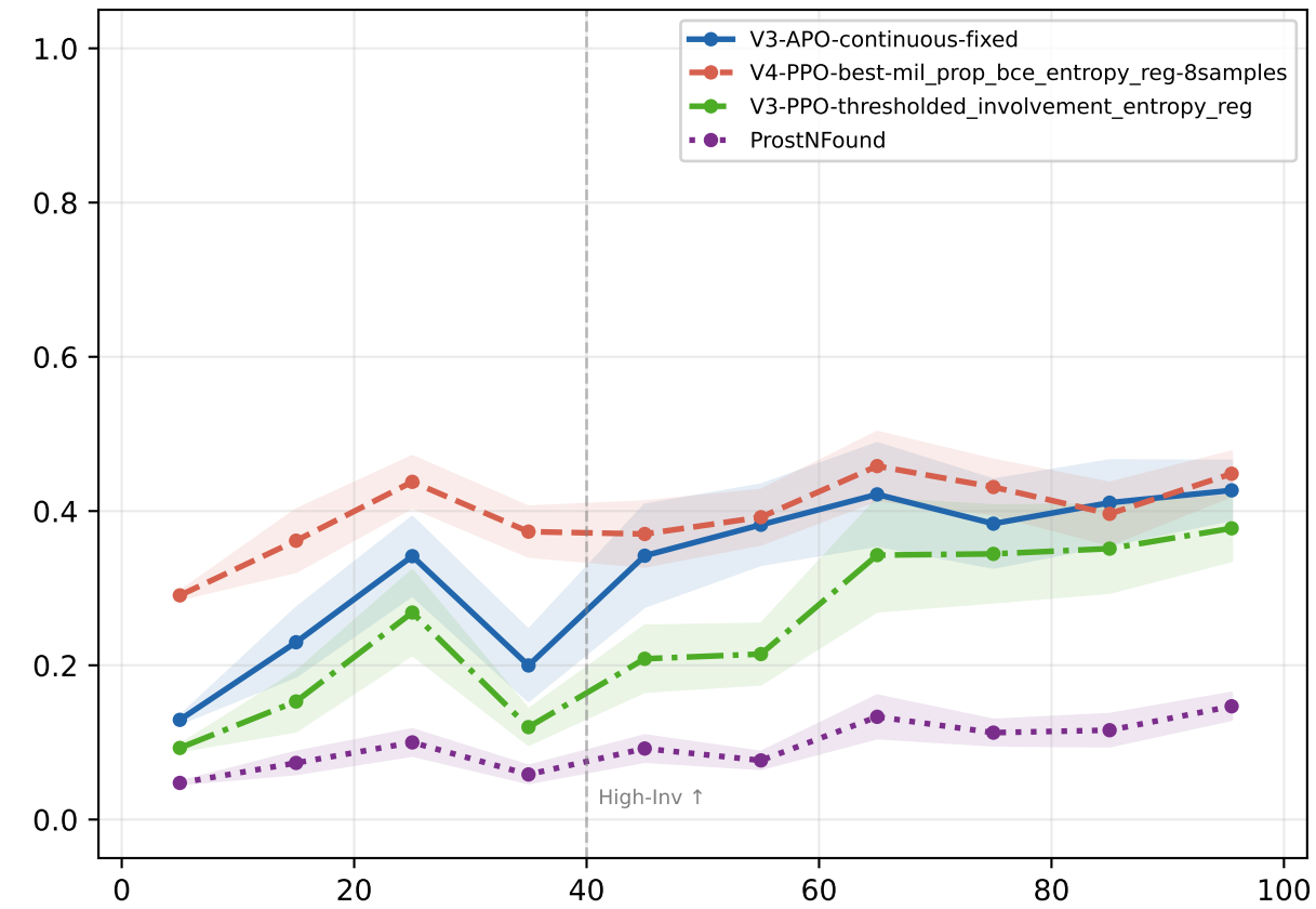
Classification Head (Continuous)
