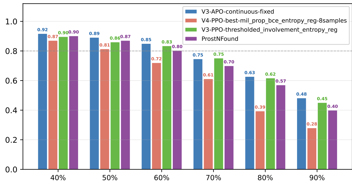
High-Involvement (>40%) Classification Head
