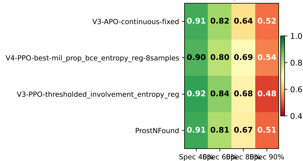
High-Involvement (>40%) Heatmap Head
