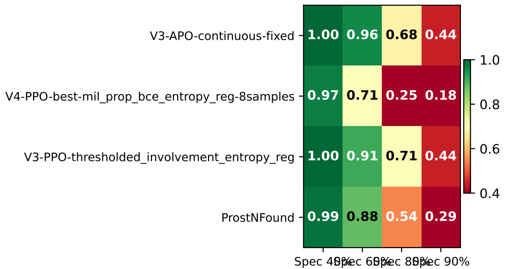
csPCa (GG ≥ 3) Classification Head
