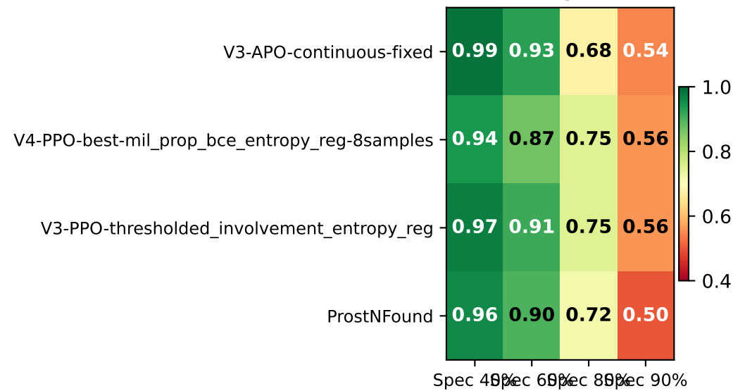
csPCa (GG ≥ 3) Heatmap Head
